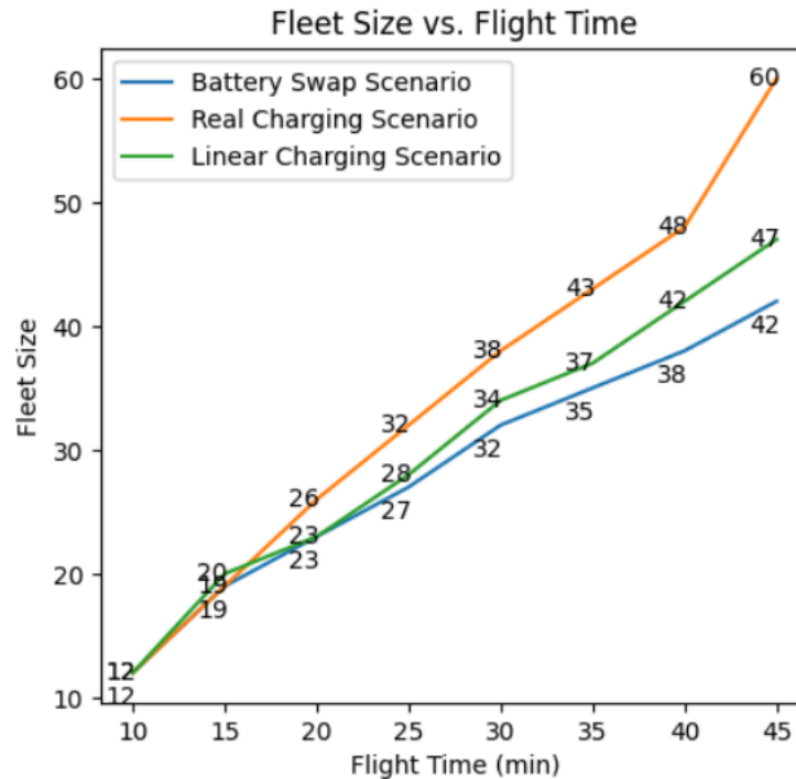
FIGURE 8: Real Charging Scenario vs Battery Swap Scenario
